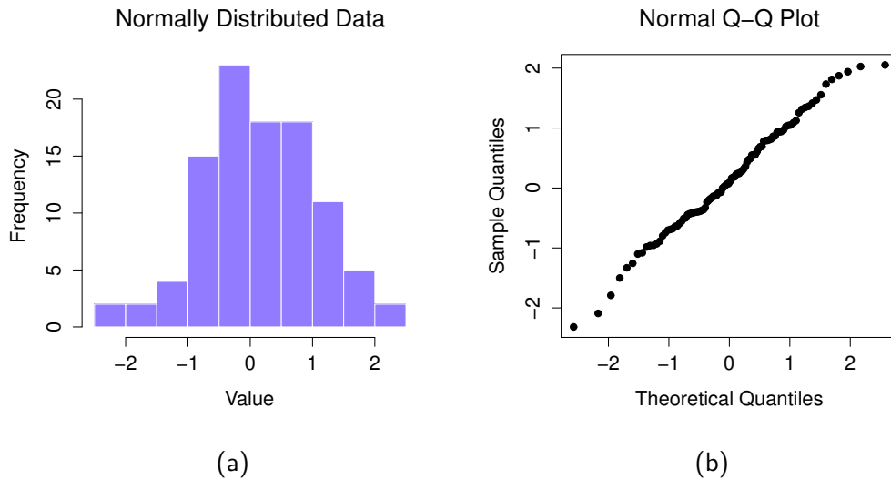
Figure 1.20 Histogram (panel a) and normal QQ plot (panel b) of normal data, a normally distributed sample with 100 observations. The Shapiro-Wilk statistic associated with these data is W = .99 , indicating that no significant departures from normality were detected ( p = .73 ).
