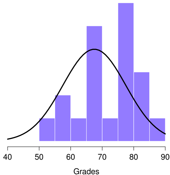
Figure1.1 The theoretical distribution (solid line) from which the psychology student grades (bars) are supposed to have been generated.
